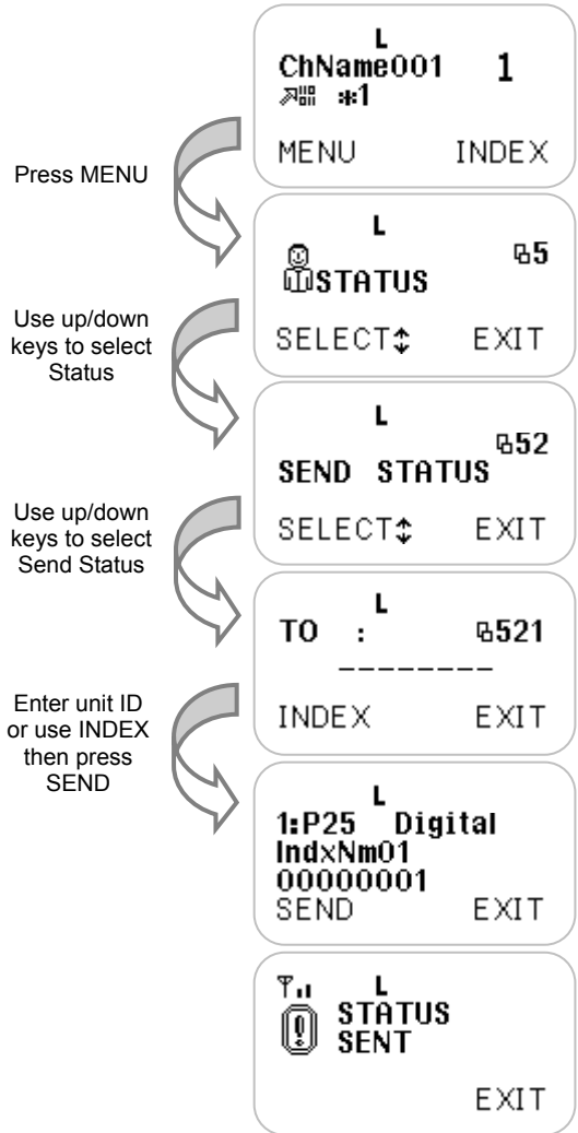
Figure 4.49 – Sending status
